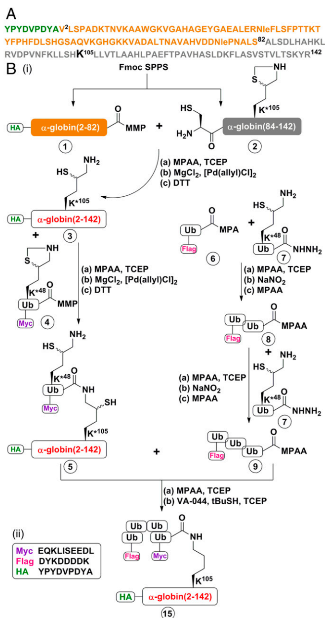
Fig. 1. Representative scheme of the strategy used for chemical synthesis of differentially tagged tetra-Ub HA-α-globin. A detailed description of the complete synthesis of the building blocks and intermediates for the generation of HA-α-globin constructs is provided in SI Appendix, Figs. S1–S23 . (A) Sequence of human HA-α-globin. The HA tag sequence is in green. The fragment 1 sequence (residues 2–82) is in light brown, and the fragment 2 sequence (residues 83–142) is in gray. Note that Ala 83 in the native α-globin was substituted with Cys to enable chemical ligation and later desulfurized back to Ala. (B, i) Chemical synthesis steps of tetra-Ub HA-α-globin (construct 15). HA-α-globin K 105 (intermediate 3; K 105 denotes the presence of δ-mercaptolysine at this position) was generated from the ligation of fragments 1 and 2 of α-globin. Note that native α-globin contains a Cys residue at position 105. The ubiquitination sites of globins have not been identified; a previous study reported successful ubiquitination at position 105, generating a thiolester bond on the native Cys residue (15). In the present study, to generate an isopeptide bond, the native Cys residue was replaced with δ-mercaptolysine. Intermediate 3 was next ligated with (intermediate 4) Myc-Ub(K 48 )-MMP; K 48 denotes the presence of δ-mercaptolysine at this position) to obtain intermediate 5, which contains the whole HA-α-globin to which one Myc-Ub moiety is bound. In parallel, Flag-tri-Ub-MPAA (intermediate 9) was assembled from Ub monomers. Intermediates 5 and 9 were then ligated and desulfurized to obtain the final Flag-Ub-Ub-Ub-Myc-
